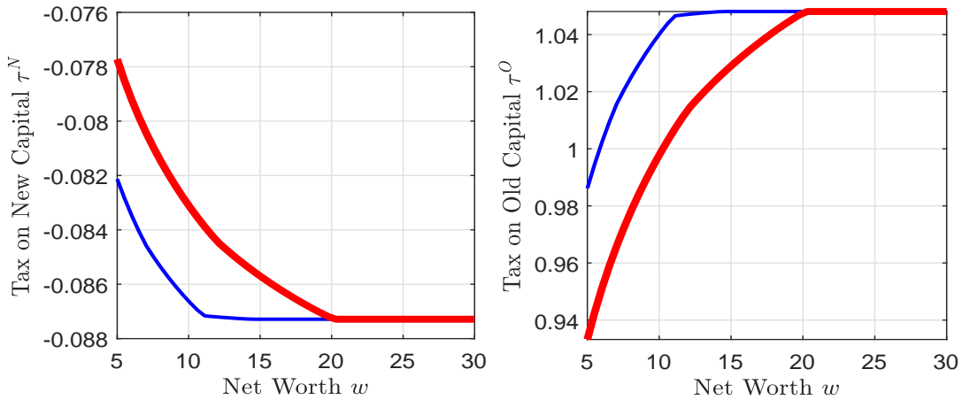
Figure OA2: Optimal tax rates. Left panel: tax rate on new capital (a negative value denotes a subsidy); right panel: tax rate on old capital. The x -axes report net worth w . Thick red lines refer to the high productivity state; thin blue lines refer to the low state. See Table 1 for the parameter values.
